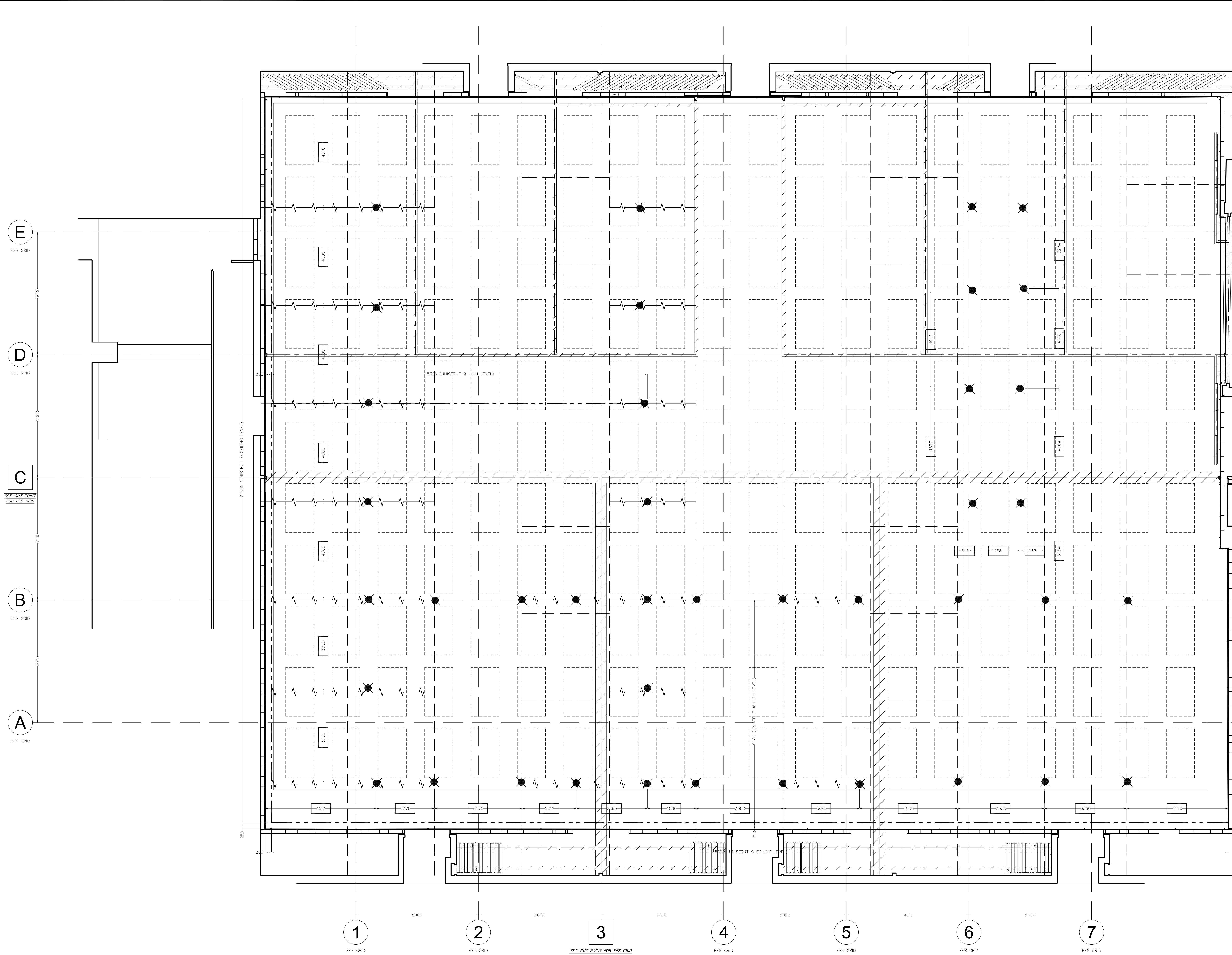
1 LIGHTING/AV HANGING POINT SET-OUT PLAN Scale: 1:50
